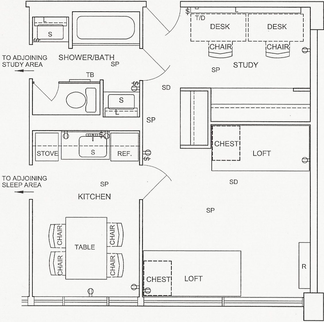
FLOOR PLAN
